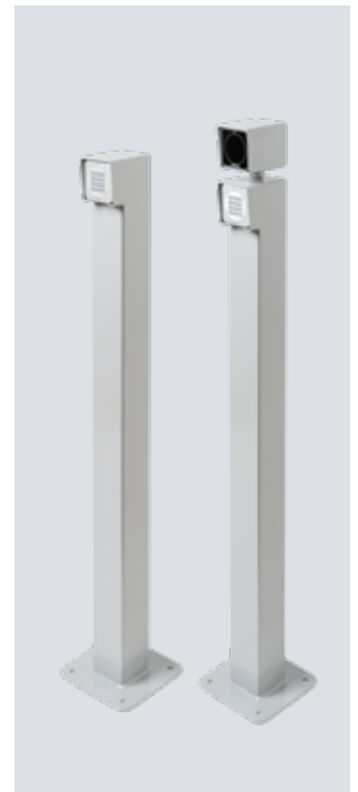
Key switch posts With a screw base for fitting to the floor, surface finish in White aluminium RAL 9006, 90 x 90 mm tube, also available as a set-in-concrete version
